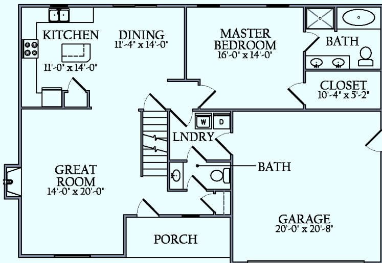
FIRST FLOOR PLAN (Dimensions Approximate)
