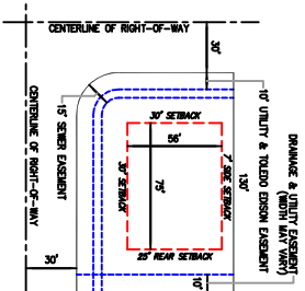
TYPICAL CORNER LOT
