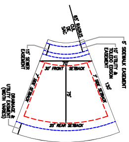
TYPICAL CUL-DE-SAC LOT
